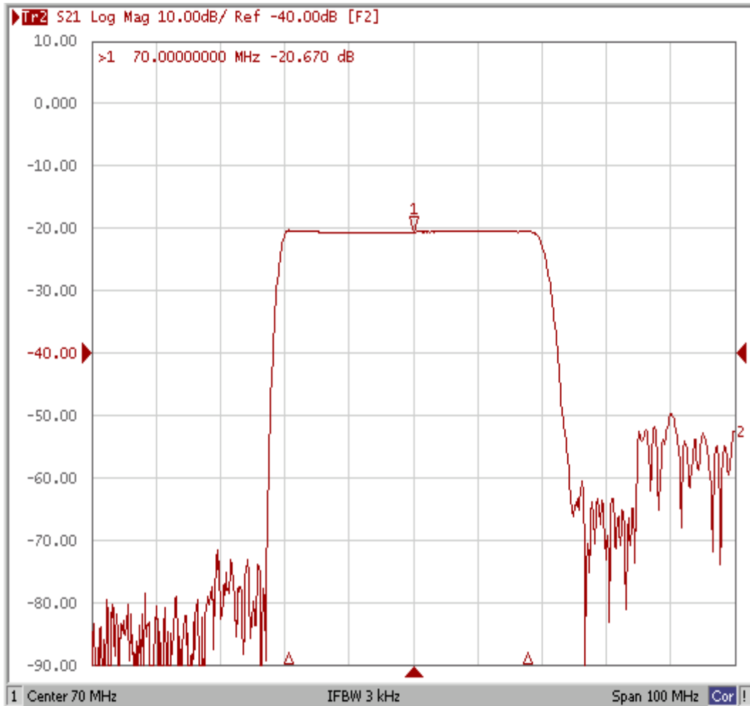
Frequency Response
